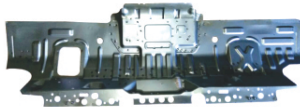
FATK 164 EC Center Flooring Assy. Complete
